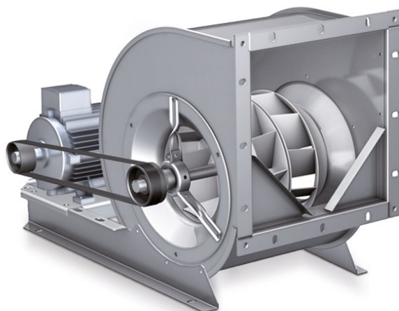
Cabinet fan with belt drive
